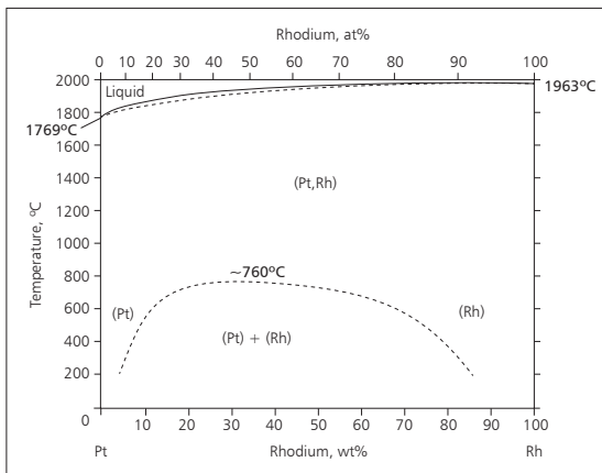
Platinum-rhodium phase diagram
