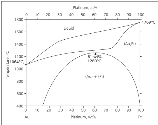
Platinum-gold phase diagram
