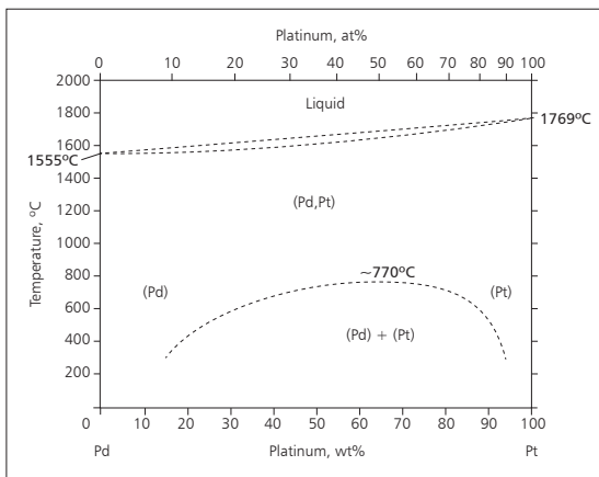
Platinum-palladium phase diagram
