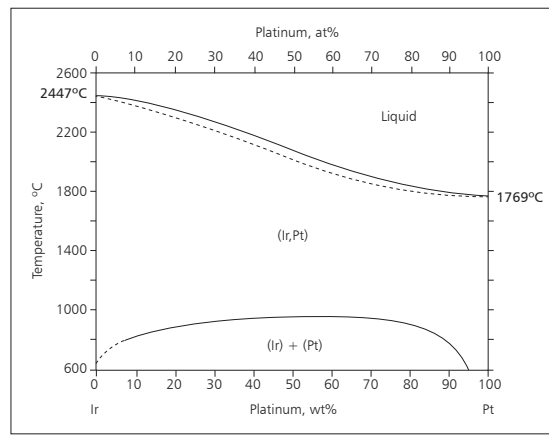
Platinum-iridium phase diagram
