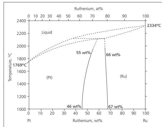
Platinum-ruthenium phase diagram
