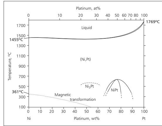
Platinum-nickel phase diagram
