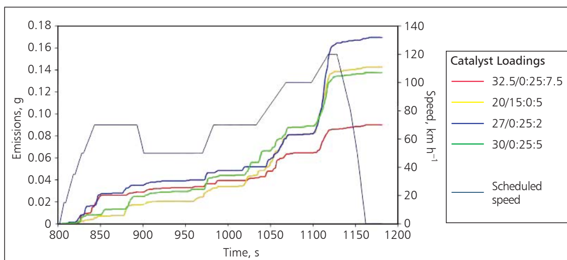
Fig. 1. Normalised EUDC NOx emissions for Set 2 catalysts, showing a clear effect of rhodium loading
